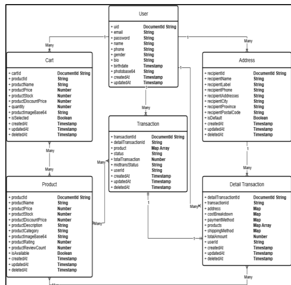
Figure 6. Class Diagram dan Entity Relationship Diagram
